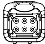
PIN/MALE CONTACT CAVITY IDENTIFICATION ON REAR
